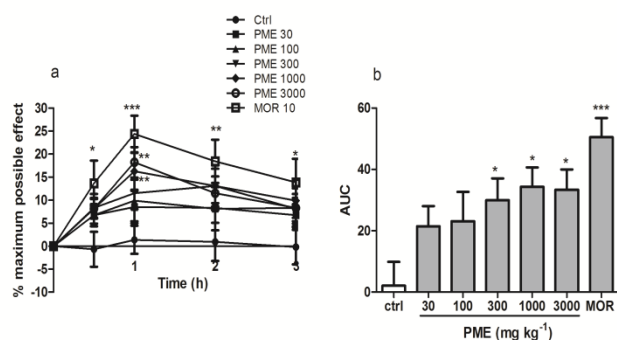
Figure 6: Effect of PME (30-3000 mg kg -1 , p.o. ) and morphine (10 mg kg -1 , i.p. ) on the time course curve (a) of the tail immersion test and the AUC (b) in mice. Data are presented as mean ± S.E.M. * P <0.05; ** P <0.01; *** P <0.001 compared to vehicle-treated group (Two-way ANOVA followed by Bonferroni's post hoc test for time course curve or one-way ANOVA followed by Newman-Keuls post hoc test for AUC).
